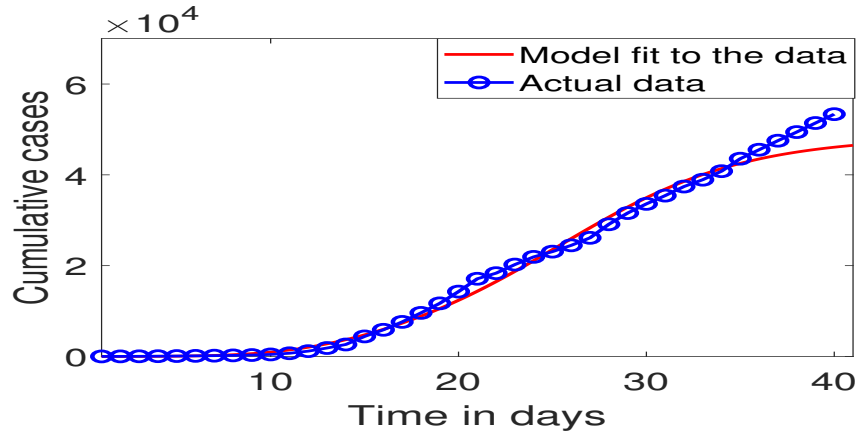
Figure 2: Simulation results showing the model estimates versus the observed cases.
